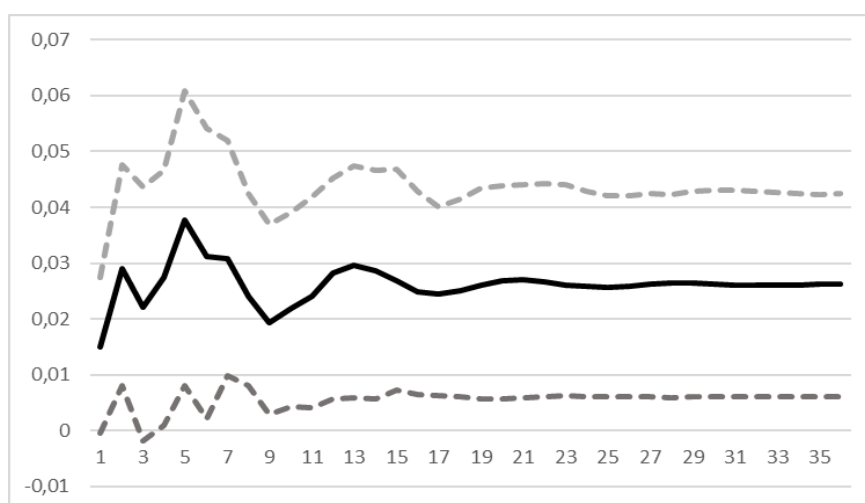
Figure 4: Accumulated response of private investment to a standard deviation shock in public investment in the linear VAR using the exchange rate variable as exogenous
