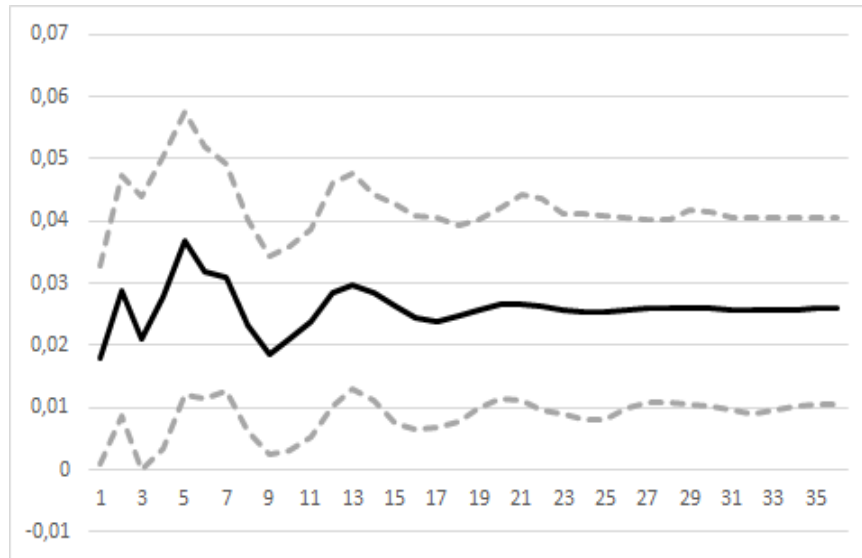
Figure 1: Accumulated response of private investment to a standard deviation shock in public investment in the linear VAR
