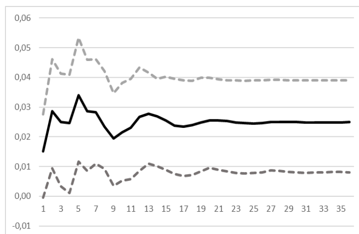
Figure 3: Accumulated response of private investment to a standard deviation shock in public investment in the linear VAR using the capacity utilization variable as exogenous
