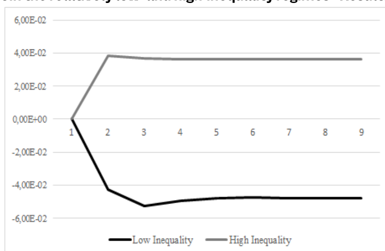
Figure 1C: Accumulated response of public investment to a standard deviation shock in private investment in the relatively low- and high-inequality regimes - Results from TVAR
