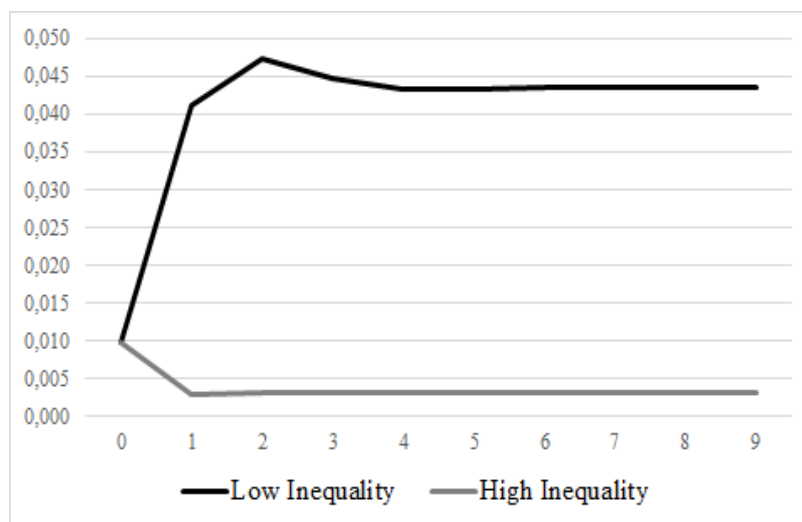
Figure 2: Accumulated response of private investment to a standard deviation shock in public investment in relatively low- and high-inequality regimes
