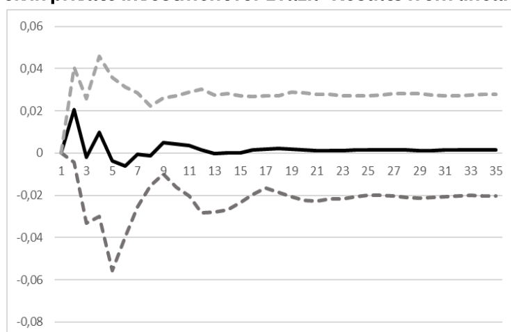
Figure 2C: Accumulated response of public investment to a standard deviation shock in private investment for Brazil - Results from linear VAR
