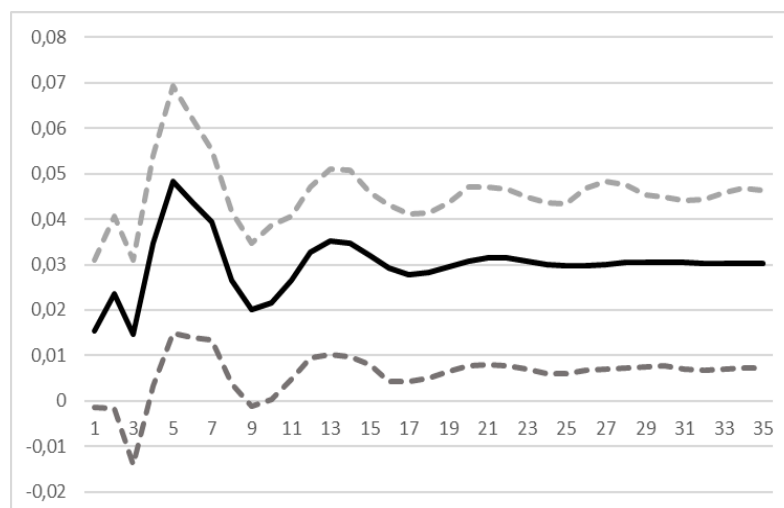
Figure 5: Accumulated response of private investment to a standard deviation shock in public investment in the linear VAR using the commodities variable as exogenous
